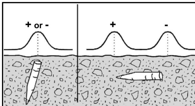
Figure 26: Basic signal patterns from vertical and horizontal targets help to determine target orientation.
