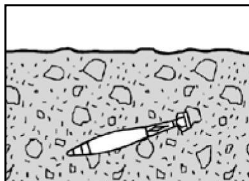
Figure 28: An 81mm mortar can be located up to 14 inches deep.
